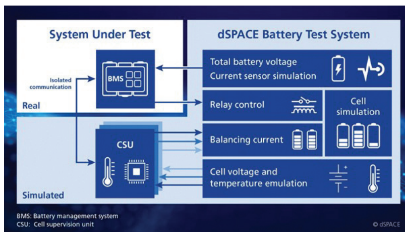
Figure 2. Diagram of battery cell, CSU and communication with the main BMS controller simulation when using the dSPACE solution for signal-level BMS testing
