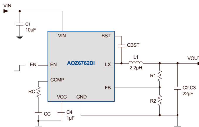
Figure 1. 2A Synchronous Buck Regulator, F_s = 1.25 \text{ MHz}
