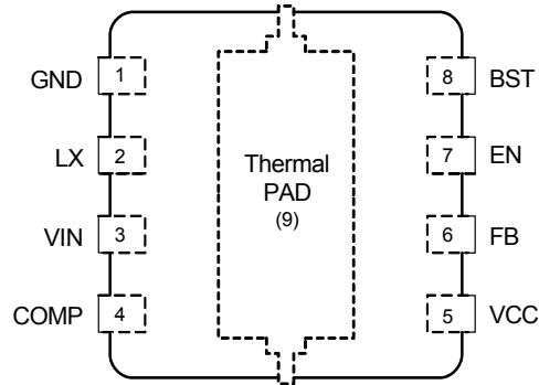
8-Pin 3mm x 3mm DFN
