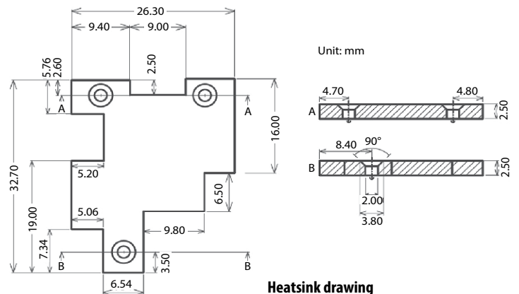
Figure 8: Heatsink attachment
