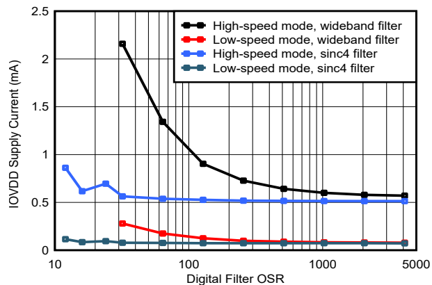
Figure 6-61. Power-Supply Current vs Oversampling Ratio
