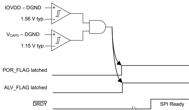
Figure 8-21. Digital Supply Threshold
