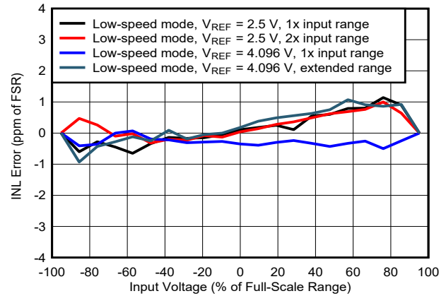
Figure 6-43. INL Error vs Input Voltage
