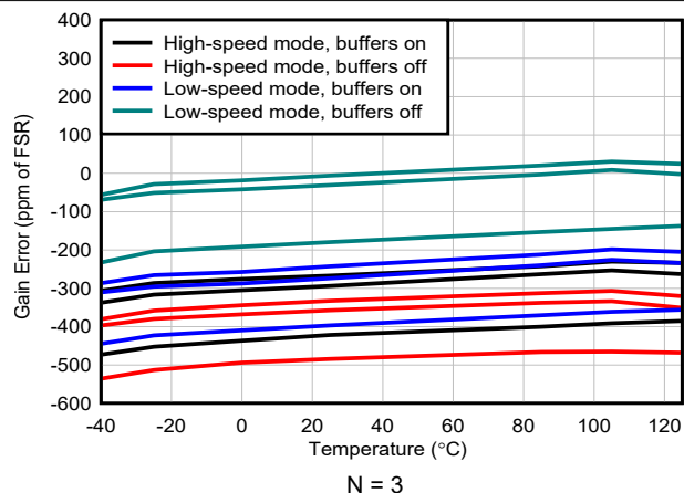
Figure 6-37. Gain Error vs Temperature
