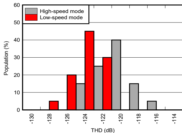
Figure 6-40. THD Distribution
