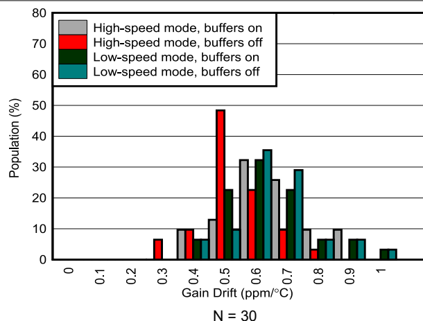
Figure 6-39. Gain Drift Distribution
