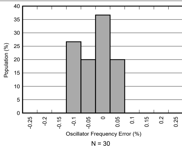
Figure 6-50. Oscillator Frequency Distribution
