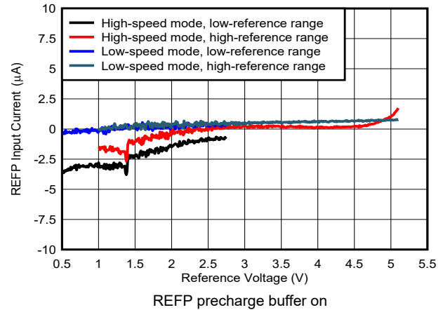
Figure 6-55. REFP Input Current vs Reference Voltage
