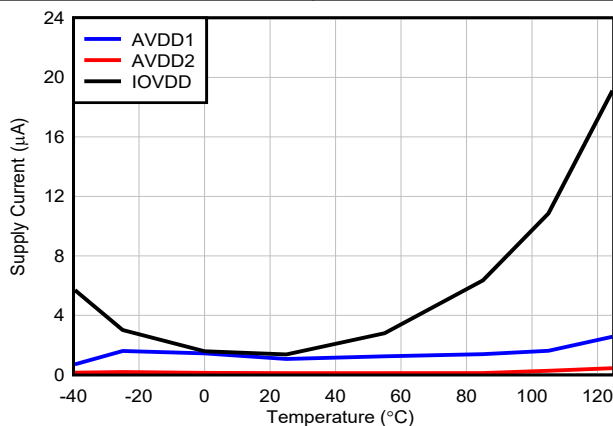
Figure 6-60. Power-Supply Current vs Temperature
