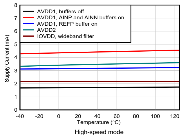
Figure 6-59. Power-Supply Current vs Temperature
