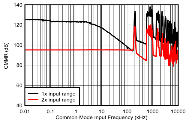
Figure 6-48. CMRR vs Frequency
