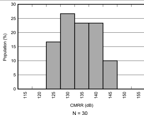
Figure 6-46. DC CMRR Distribution
