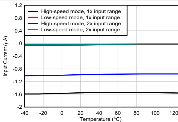
Figure 6-30. Input Current vs Temperature
