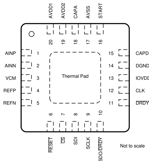
Figure 5-2. RUK Package (Preview), 20-Pin WQFN (Top View)
