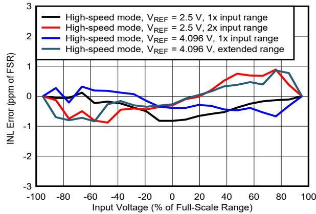
Figure 6-42. INL Error vs Input Voltage
