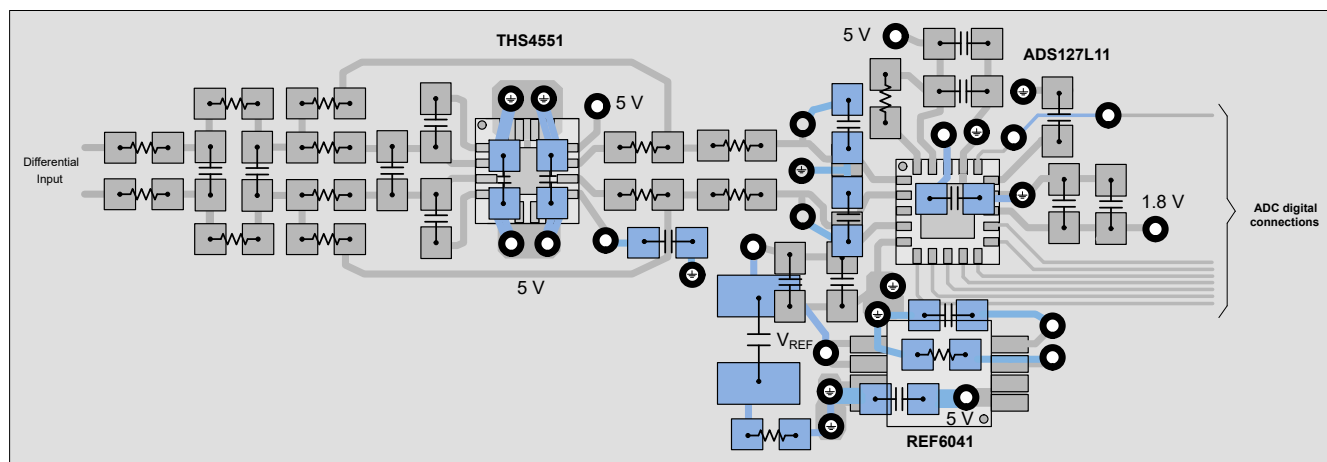
Figure 11-1. Layout Example of Typical Application Circuit
