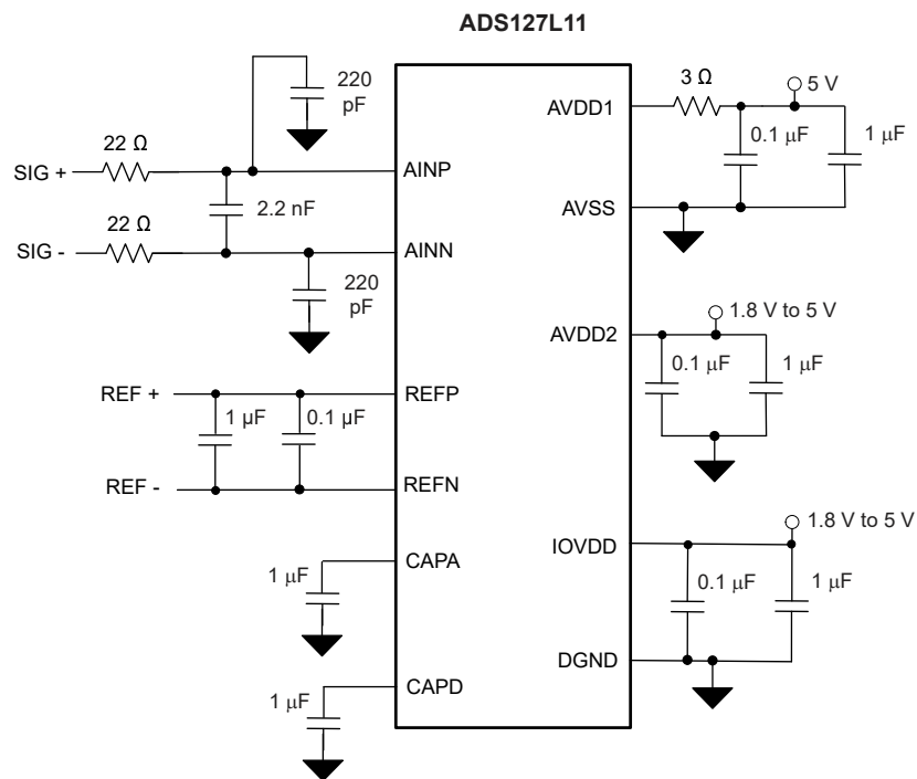
Figure 10-1. Device Bypass Recommendation
