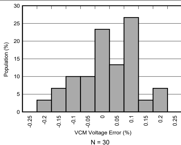
Figure 6-52. VCM Voltage Distribution
