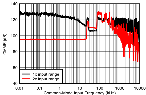
Figure 6-49. CMRR vs Frequency
