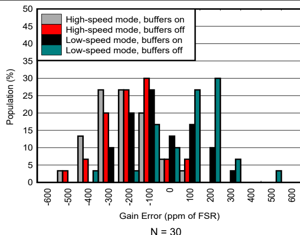
Figure 6-36. Gain Error Distribution
