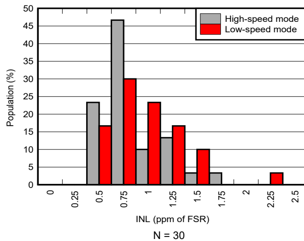
Figure 6-44. INL Distributions
