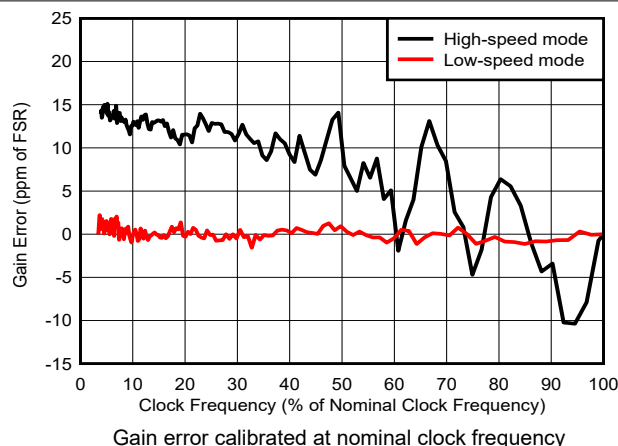
Figure 6-38. Gain Error vs Clock Frequency
