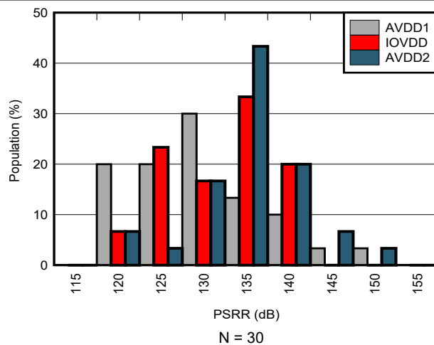
Figure 6-56. DC PSRR Distribution
