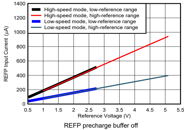
Figure 6-54. Reference Input Current vs Reference Voltage
