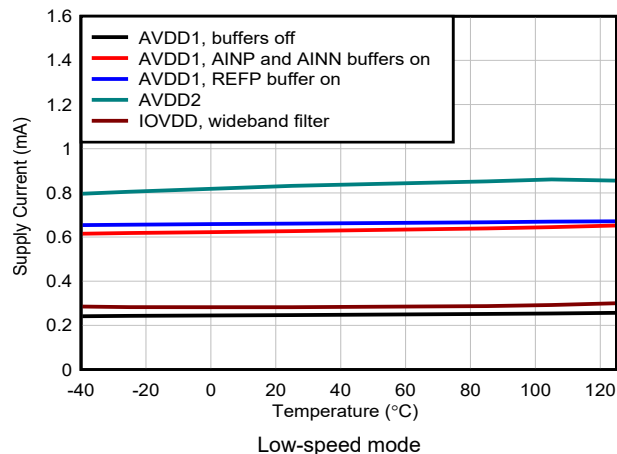
Figure 6-60. Power-Supply Current vs Temperature
